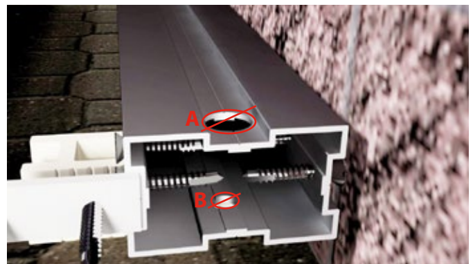
26. Different-diameter holes in the batten.
