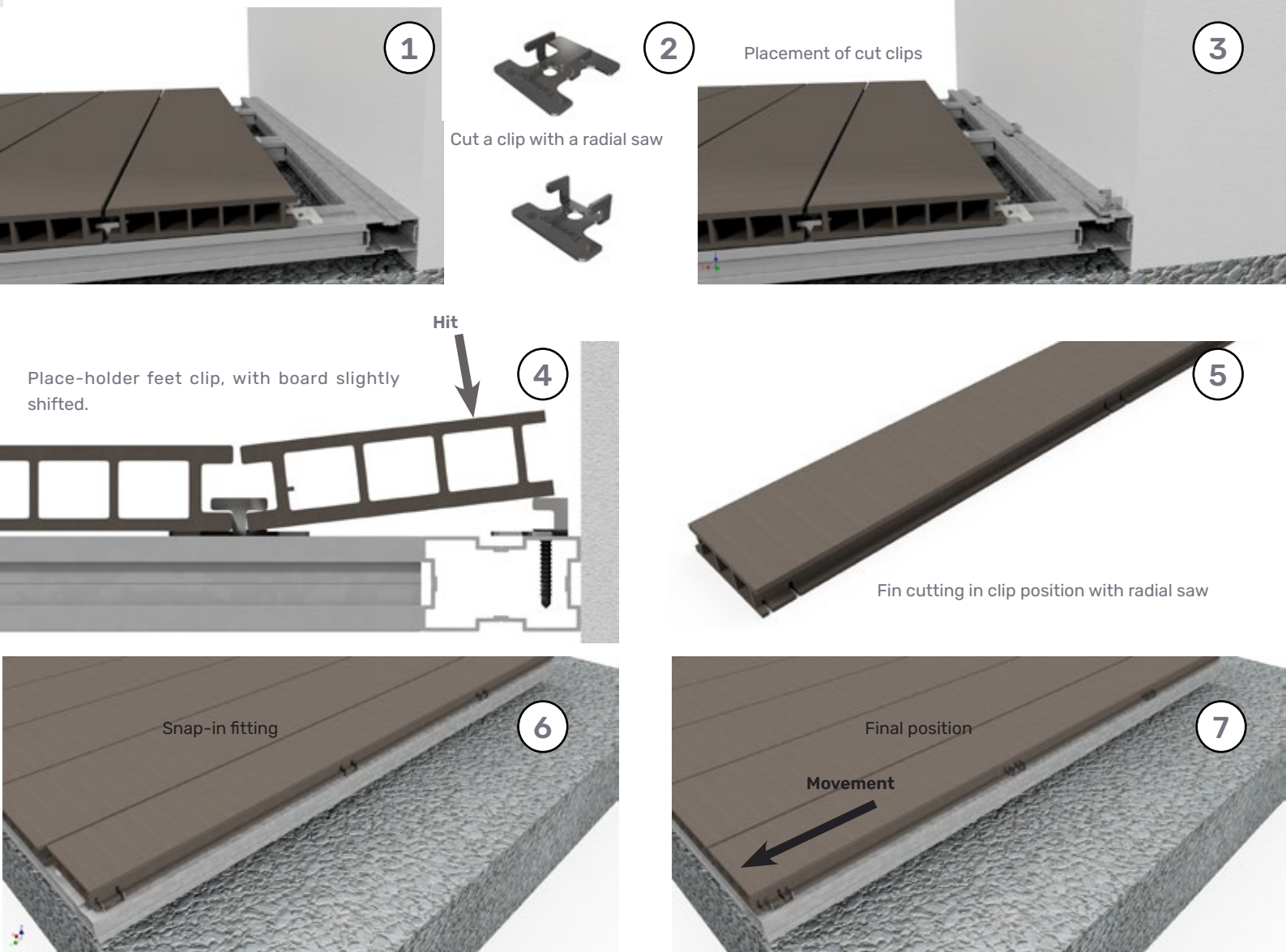
47. Hidden fixing sequence with clip.
