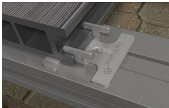
17. Details of slat fixing with a clip
