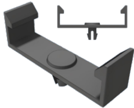
9. Batten-plot anchor clip.
